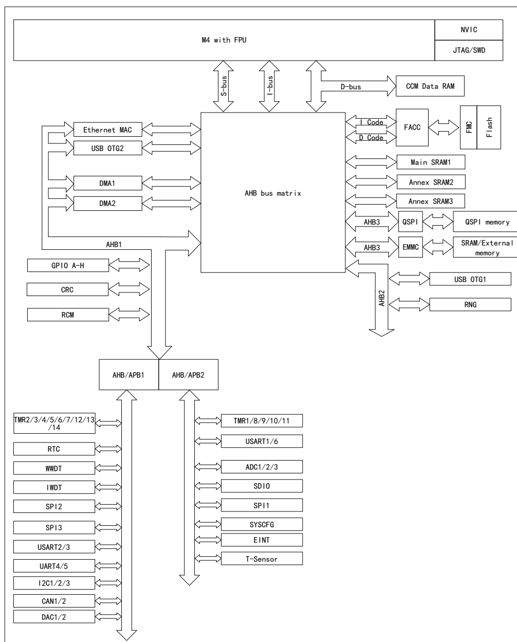
Figure 1 APM32F427xG_F425xG_F423xG System Architecture Block Diagram
