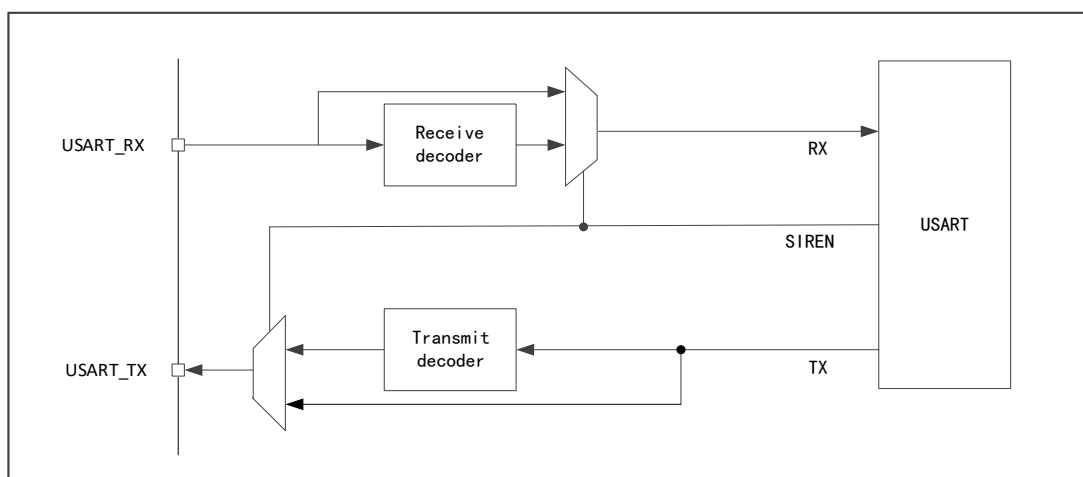
Figure 75 IrDA Mode Block Diagram
