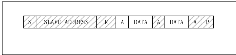
Figure 81 Master Reads Data from Slave
