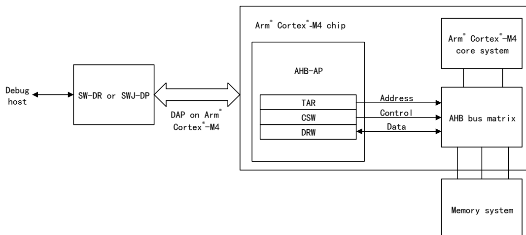
Figure 12 APM32F427xG_F425xG_F423xG Level and Arm® Cortex® -M4F Level Debugging Block Diagram
