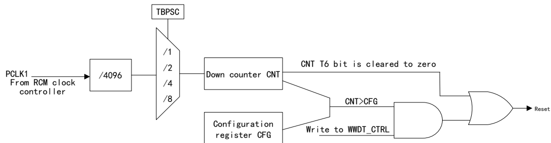
Figure 64 Window Watchdog Structure Block Diagram
